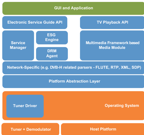
Aricent Mobile TV Architecture
